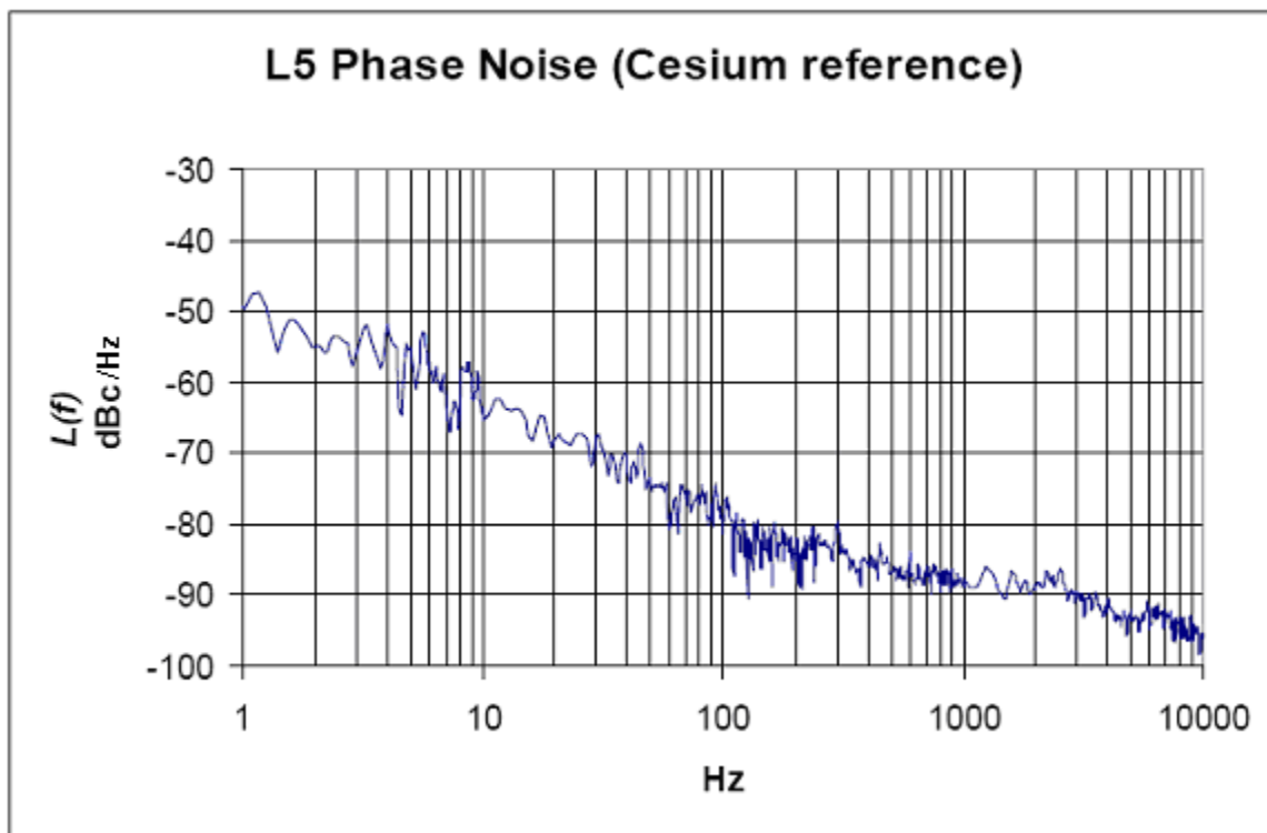
Figure 6-1. Carrier Phase Noise Spectral Density
