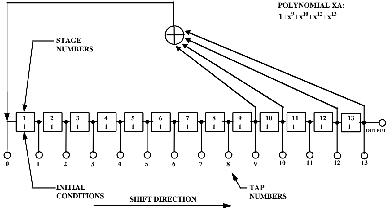
Figure 3-4. XA Shift Register Generator Configuration.
